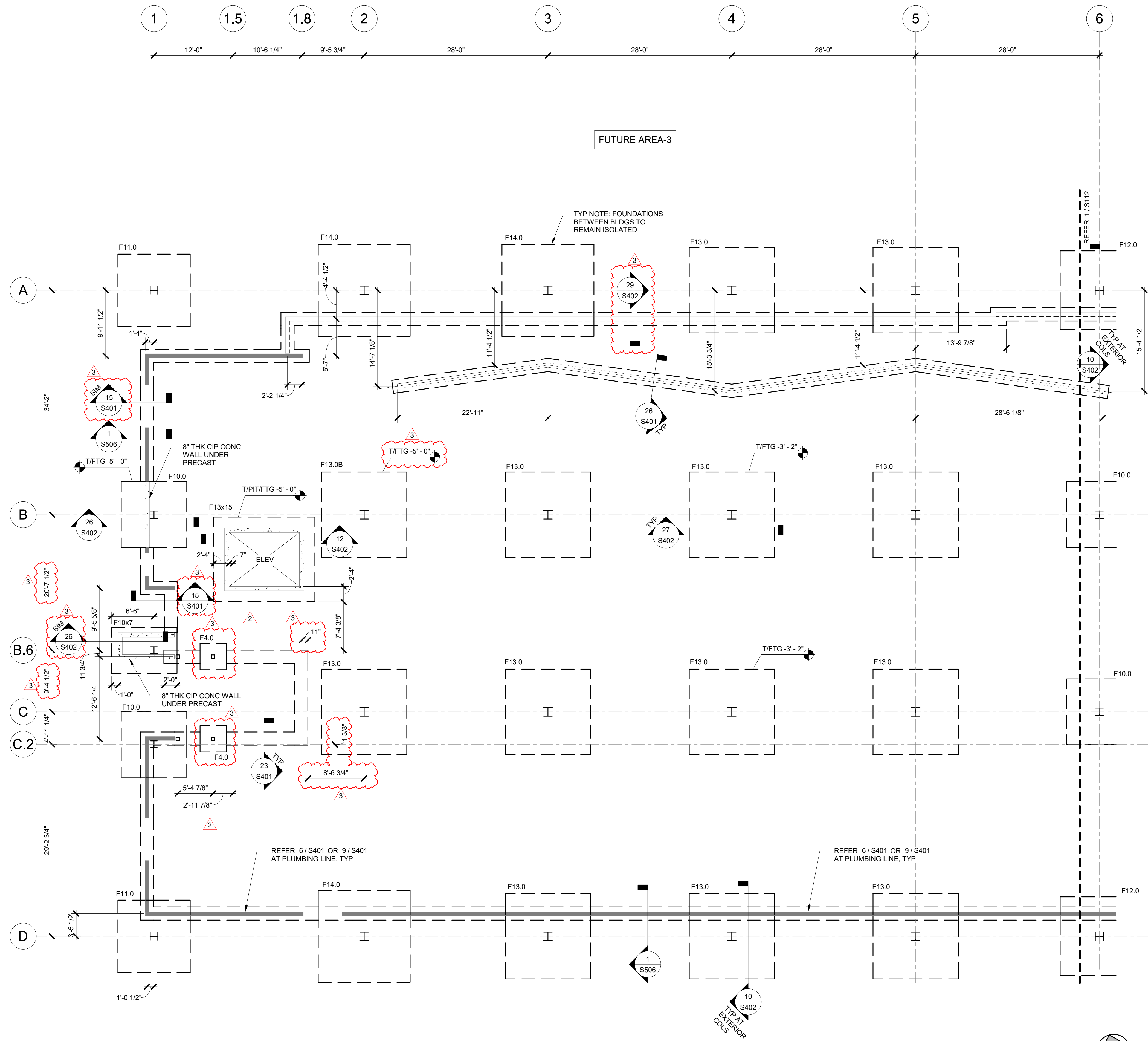
1 FOUNDATION PLAN AREA 1 1/8" = 1'-0"
